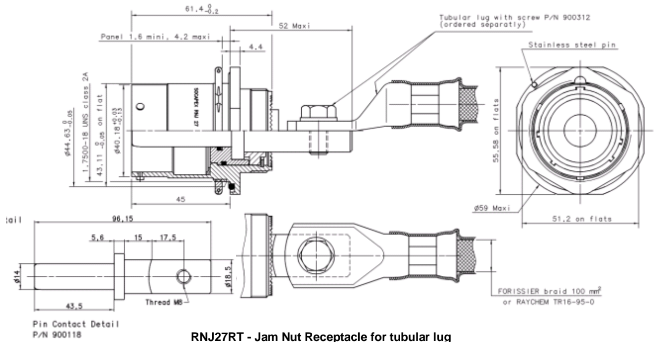
RNJ27RT - Jam Nut Receptacle for tubular lug
