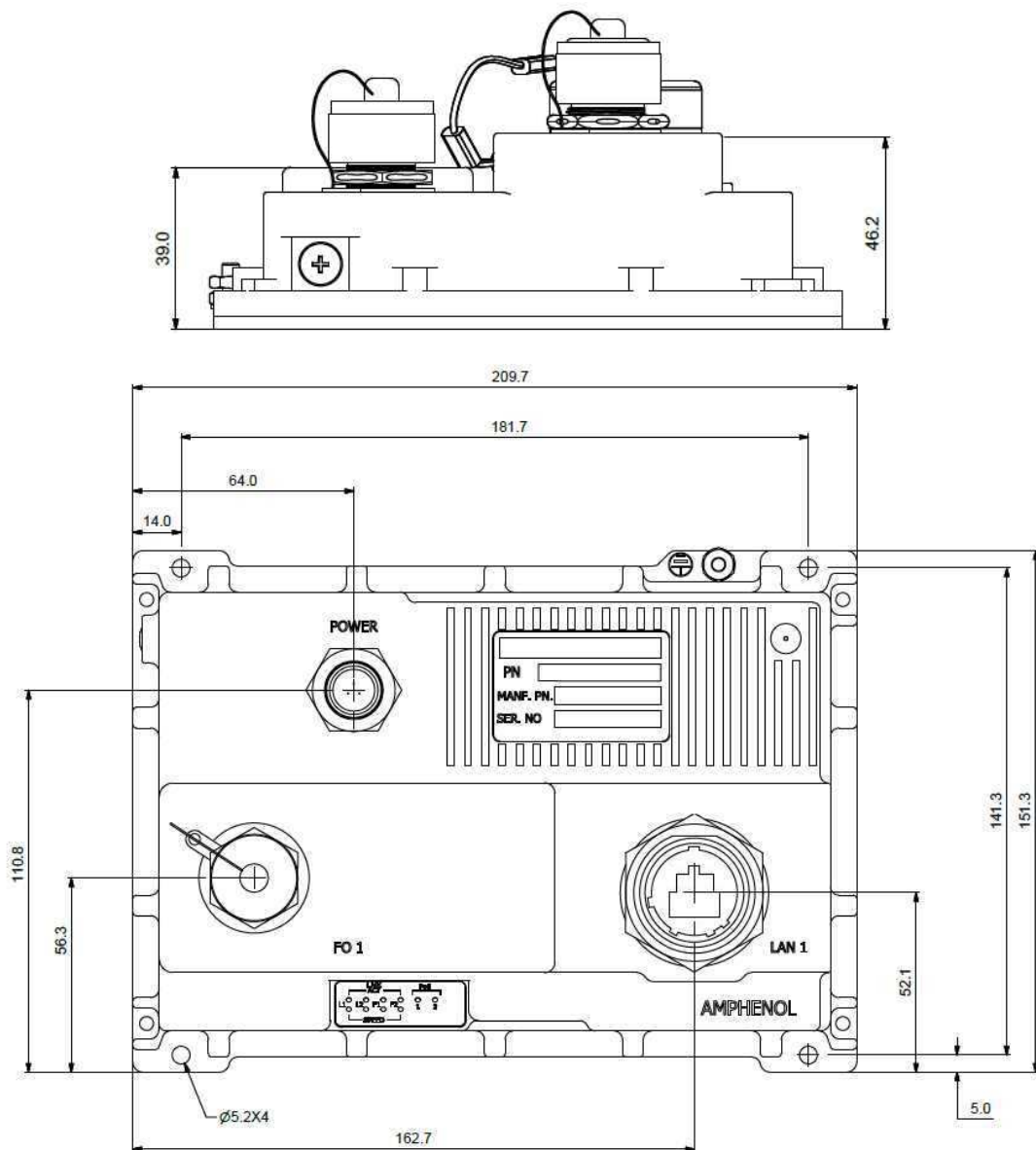
Figure 2 : RES-GMC Physical Dimensions
