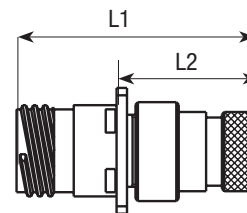
Startop Square Flange Receptacle with backshell for pigtails STA 00 R VX XX X XXXX XX CXXX
