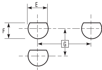
Panel Drilling for Jam Nut receptacle
