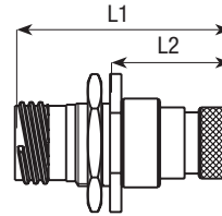
Startop Jam Nut Receptacle with backshell for pigtails
