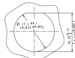
Panel drilling
