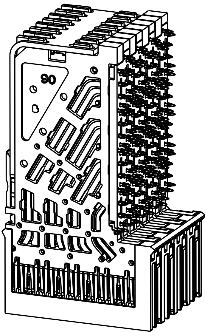
ISOMETRIC VIEW COMPLIANT GUIDE FULLY SEATED SCALE 4/1
