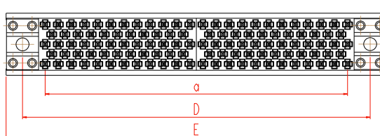
116 signal contacts
