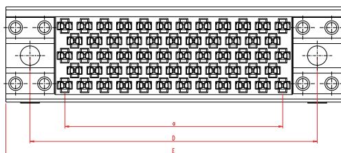
58 signal contacts
